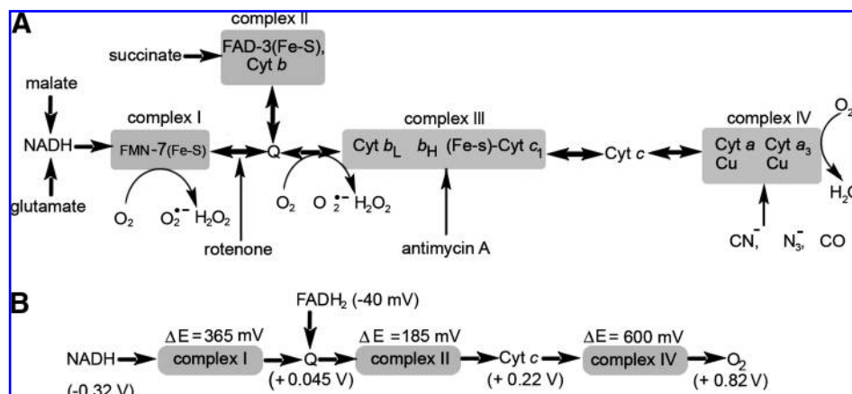
FIG. 2. (A) Sites of O_2^{\bullet -} generation along electron-transport system with several respiratory inhibitors. (B) Diagram of electron-transport system with standard reduction potentials ( E^{\circ} ) of mobile components and \Delta E^{\circ} where sufficient free energy is harvested to synthesize ATP.
